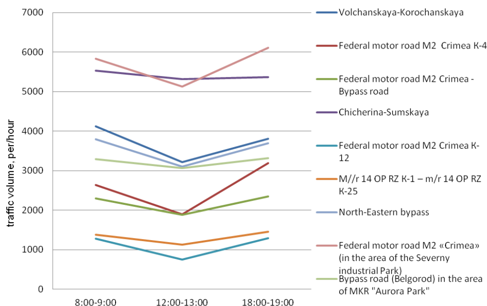
Figure 2: Traffic volume on the studied objects during the rush hour
