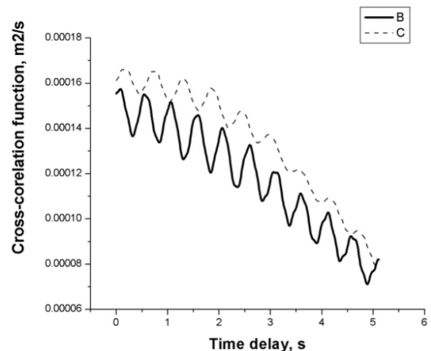
Figure 5: Cross-correlation function
