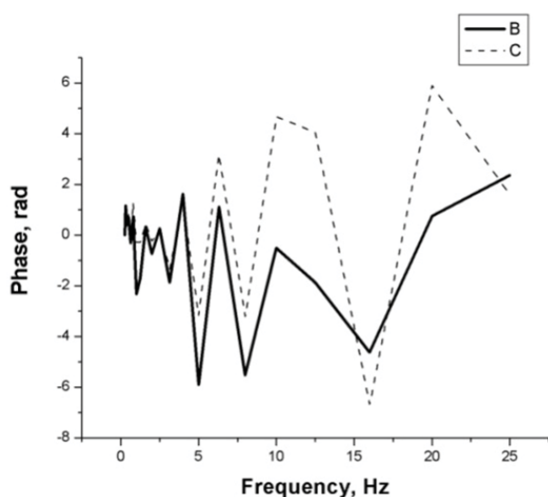
Figure 7: Phase angle of transfer function
