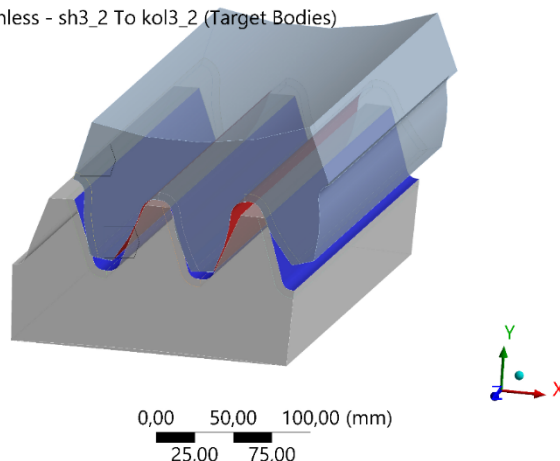
Fig. 3. Contact between the tooth profiles of the gear and the wheel
