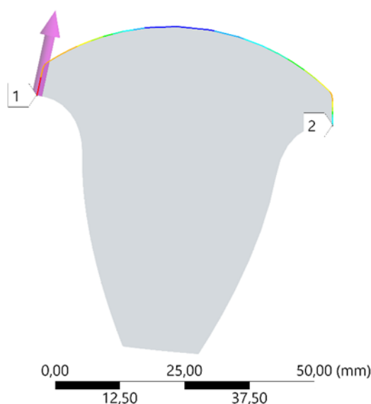
Fig. 13. Bending stress at the junction of the clad tooth
