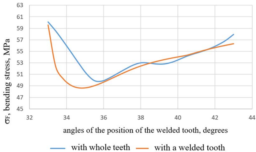
Fig. 16. Results of the bending stress calculation
