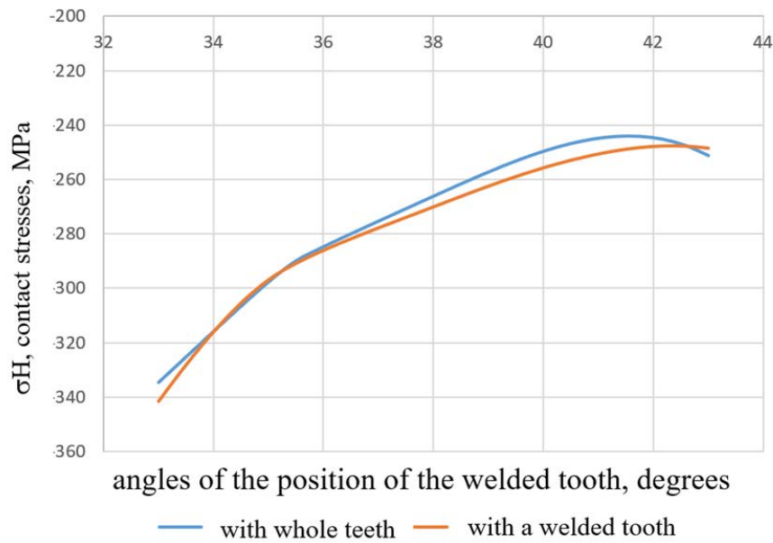
Fig. 15. Results of the contact stress calculation
