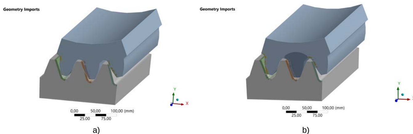
Fig. 2. Three-dimensional model of a gear pair: a) with solid teeth; b) with a clad tooth
