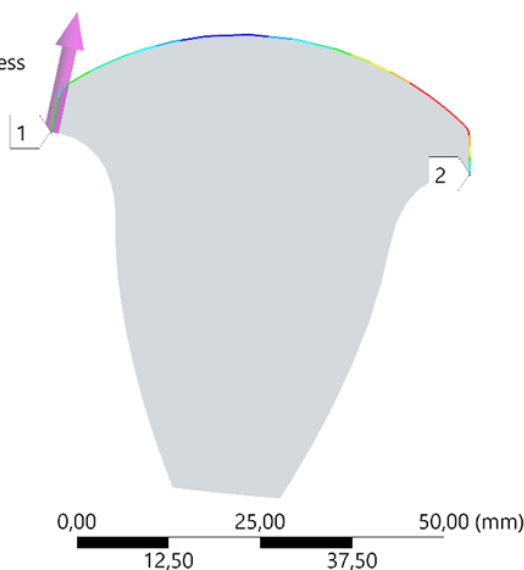
Fig. 12. Stress along the Misese at the junction of the clad tooth
