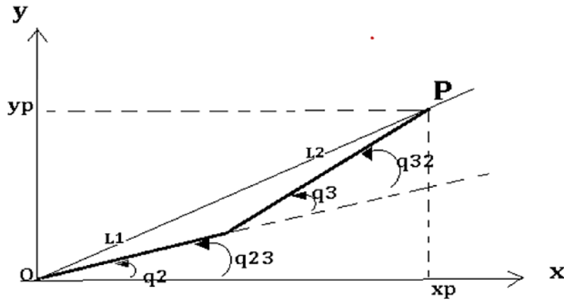
Fig. 2. Inverse kinematic diagram
