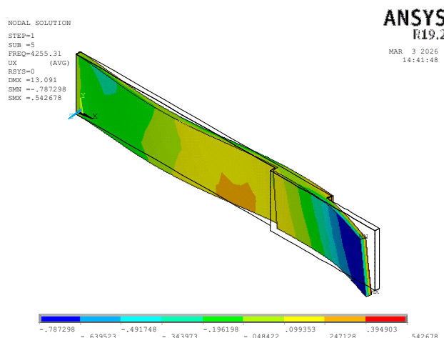
Fig. 4. Effect of bonding length on the natural frequency (Hz) and mode shape 5
