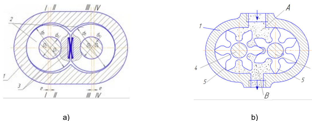
Fig. 1. Arrangement of two support bushings in the housing bores of the gear pump and the operating process: a) arrangement of two support bushings in the housing bores of the gear pump; b) operating process
