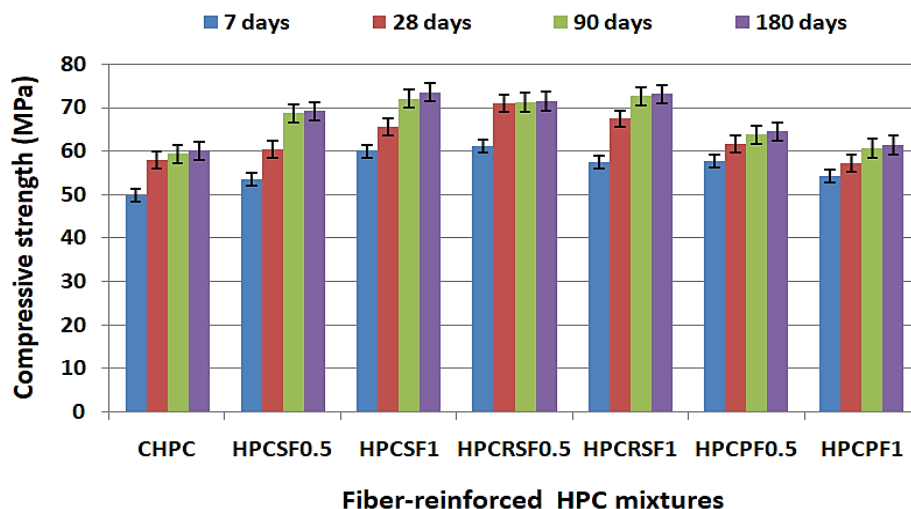
Fig. 7. Compressive strength of fiber-reinforced HPC mixtures
