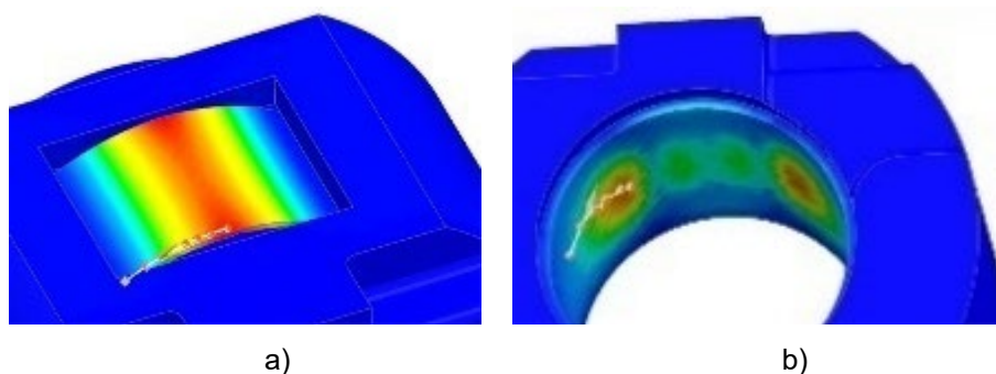
Fig. 12. Segments of the measurement results of the loads acting on the plate and the effect on the bushing housing, on the basis of which graphs of the pressure effect results were constructed: a) load measurement segment – from the lower part of the plate to its middle along an arc with a radius of 17 mm over a length of 10 mm; b) load measurement segment – along an arc from the minimum reaction to the maximum reaction on the inner surface of the bushing over a length of 10 mm
