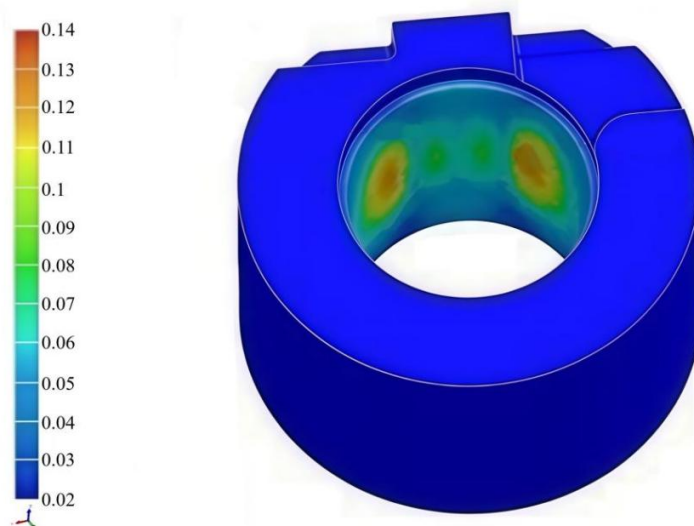
Fig. 15. Also shows a model displaying the reaction force of the plate acting on the bushing under a pressure load of 10 bar at 1000 rpm
