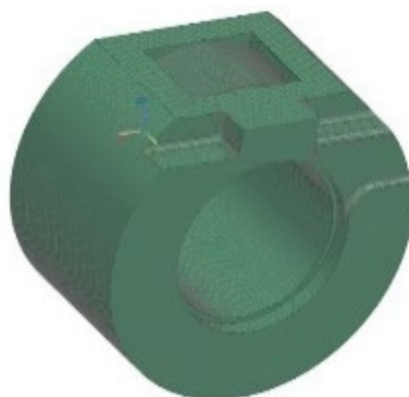
Fig. 10. FEM mesh of the support bushing with a plate
