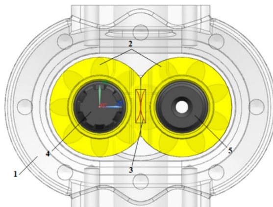
Fig. 8. Model of the gear pump with a biaxial connection with installed expanding elements: 1 – housing; 2 – bushing; 3 – elastic expanding elements; 4 – driving shaft-gear; 5 – driven shaft-gear
