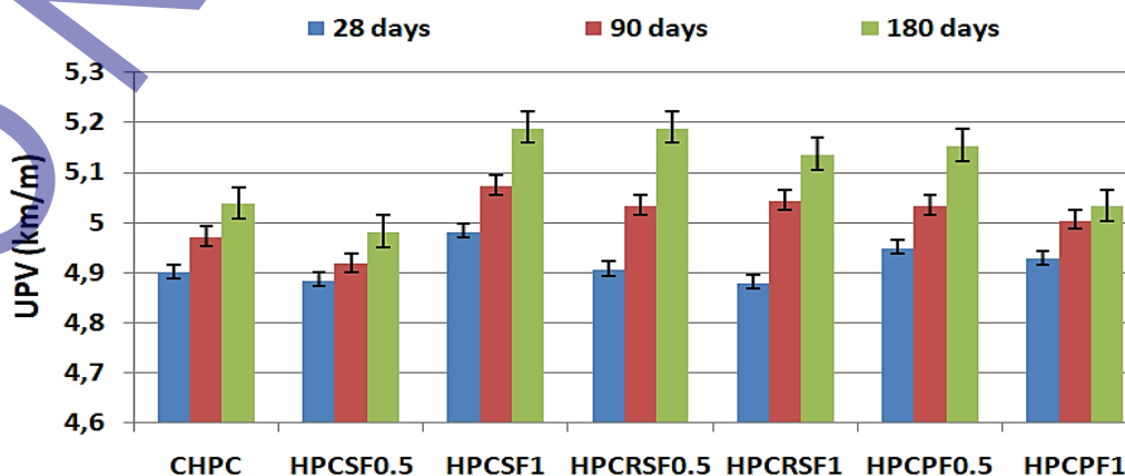
Fig. 9. UPV of fiber-reinforced HPC mixtures
