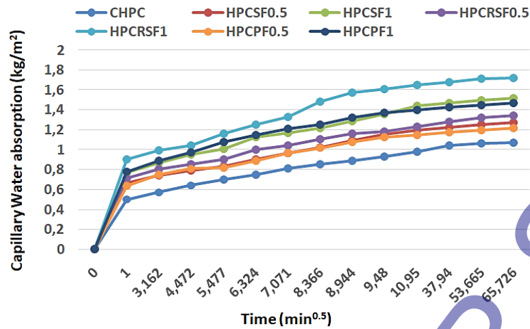
Fig. 11. Capillary water absorption of fiber-reinforced HPC mixtures
