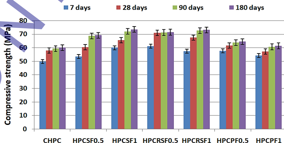
Fig. 7. Compressive strength of fiber-reinforced HPC mixtures
