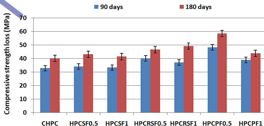
Fig. 13. Compressive strength loss of fiber-reinforced HPC mixtures immersed in HCl solution
