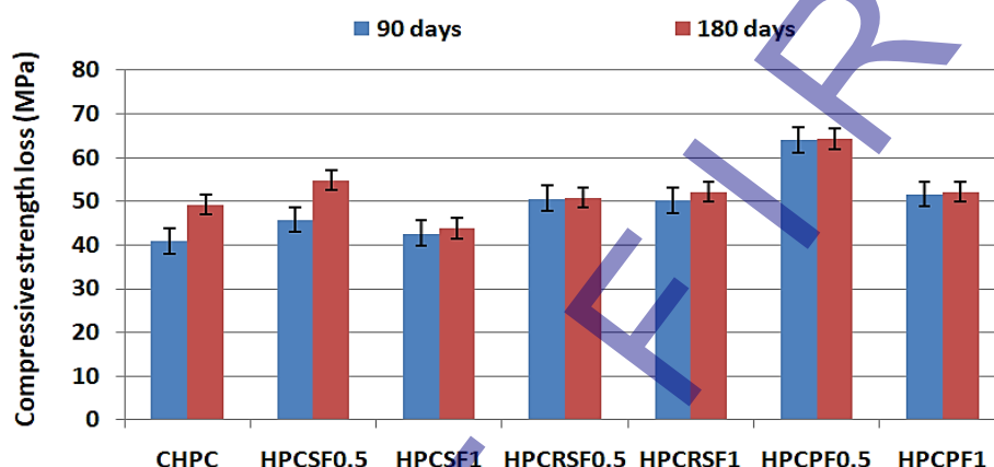
Fig. 14. Compressive strength loss of fiber-reinforced HPC mixtures immersed in H_2SO_4 solution
