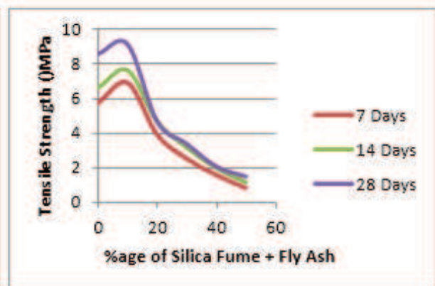
Figure 7: Strength of Cylinders made with 1:1.5:3
