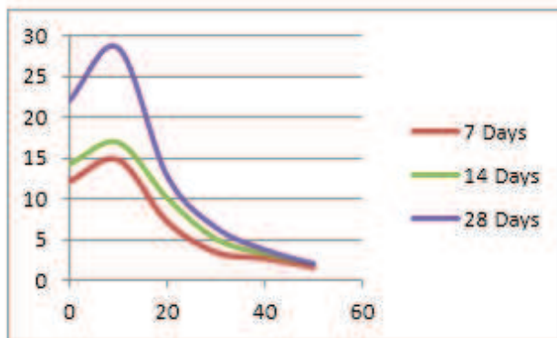
Figure 4: Strength of Cylinders made with 1:2:4 ratio
