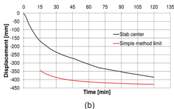
Figure 9: Relative deflection a) unprotected beam, b) central point of slab
