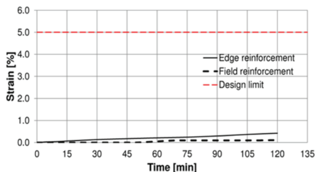
Figure 10: Plastic strains of reinforcement
